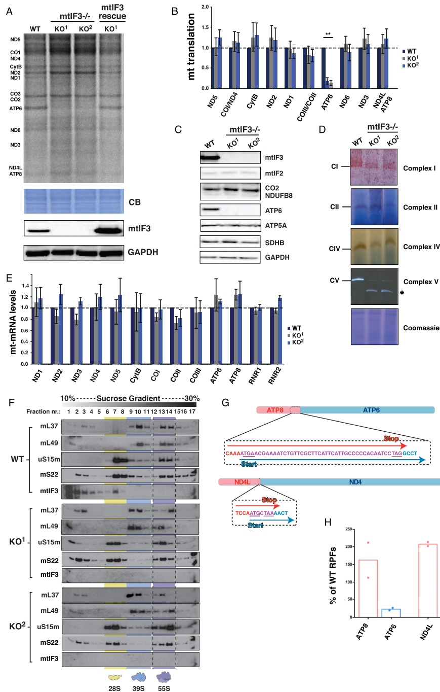
Figure 4. mtIF3 is essential for ATP6 synthesis. (A) [ 35 S]-Met/Cys labeled nascent mitochondrial polypeptides from the WT mtIF3 KO cell lines and KO 1 cells expressing mtIF3.FLAG or mtIF3-CTEΔ. Equal amounts of total proteins were separated on 12% SDS-PAGE, stained by Coomassie brilliant blue (CBB) to verify equal loading and visualized by autoradiography. mtIF3 expression is shown by the western blot with GAPDH serving as a loading control. (B) Quantification of the [ 35 S]-Met/Cys labeled mitochondrial translation products from WT and mtIF3 KO clones. Data represent mean values ± SD from 5 independent biological replicates. (C) Steady-state levels of the OXPHOS subunits from WT and mtIF3 KO cell lines were analyzed by western blot. Proteins from the whole cell lysate were resolved by SDS-PAGE and transferred to the PVDF membranes, which were then probed with the antibodies against mtIF3, mtIF2, mitochondrially-encoded (COXII, ATP6) and nuclear-encoded subunits (NDUFB8, SDHB, ATP5a) of the OXPHOS complexes. GAPDH was used as a loading control. (D) BN-PAGE analysis and in-gel staining of CI, CII, CIV and CV activities in mitochondrial protein extracts from the WT and mtIF3 KO clones. Coomassie blue stained gel is shown as a loading control. * indicates the F 1 -containing CV assembly intermediate. (E) Quantitative real-time PCR analysis of the mitochondrial mRNAs and rRNAs steady-state levels in mtIF3 KO cells relative to WT. Data is representative of the mean values ± SD from three independent experiments. (F) Mitochondrion sedimentation analyses on a sucrose density gradient (10–30%) in WT and mtIF3 KO cell lines. The yellow, blue and purple colors indicate the sedimentation of the mtSSU, mtLSU and 55S, respectively. (G) Schematics of the human mitochondrial bicistronic mRNA transcripts ATP8/ATP6 and ND4L/ND4. The overlapping sequence of the bicistrons is shown below in purple. (H) Mitochondrion profiling analysis. Percentages of mitochondrion-protected fragments (mt-RPF) per gene, relative to the WT control, shown for mitochondrial bicistronic transcripts (ATP8/ATP6 and ND4L/ND4) from mtIF3 KO 1 cells. Results represent data from two MitoRiboSeq experiments.
